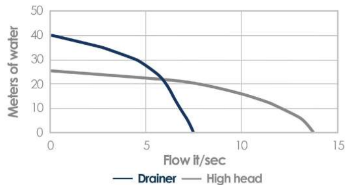
2 Inch Submersible
